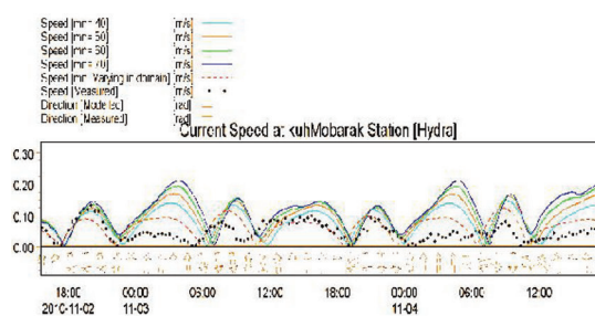
Current Speed at kuhMobarak Station [Hydra]
